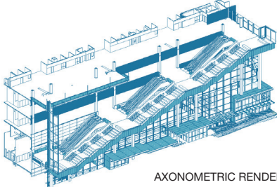
AXONOMETRIC RENDERING OF HILLCLIMB
